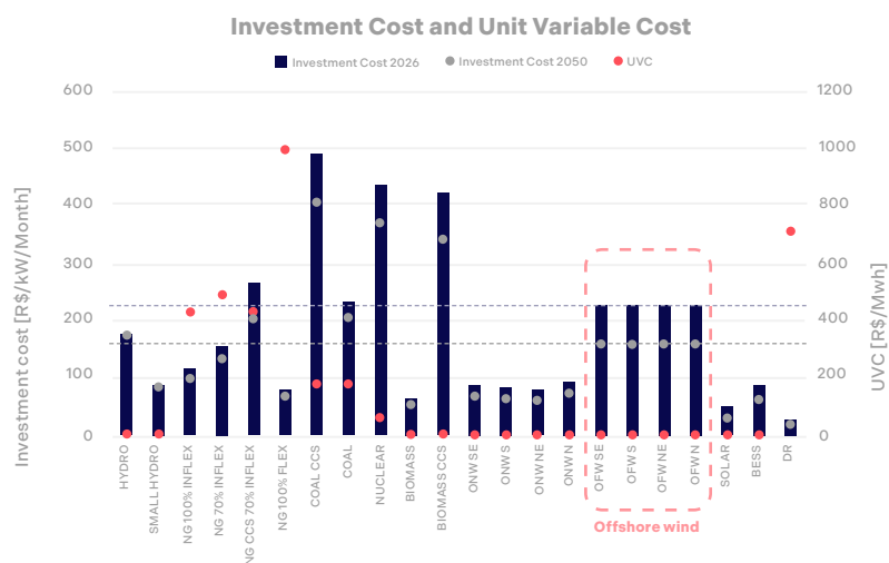
Figure 12: Investment Cost Expectations for Various Sources
